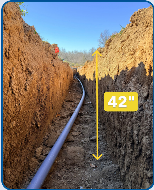
Ditch shall be 42 inches deep minimum and free from rocks/sharp objects.
